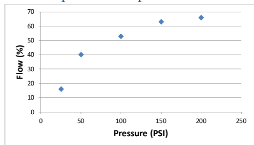
fastRise™ EZpure Flow Dependence on Pressure
