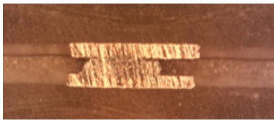
fastRise™ prepreg between subassemblies w/copper paste
