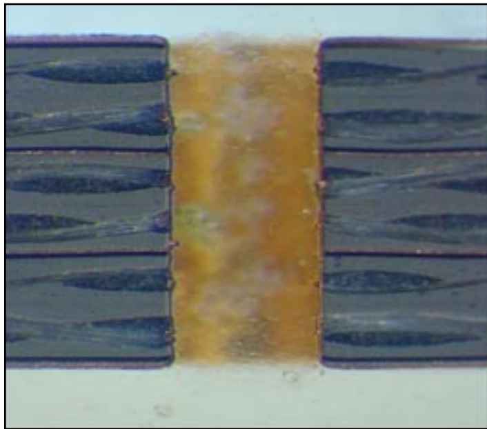
Figure 1 - Typical hole wall quality of RF-35 material
