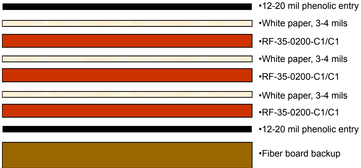
Figure 6 – Typical RF-35 rout stack-up
