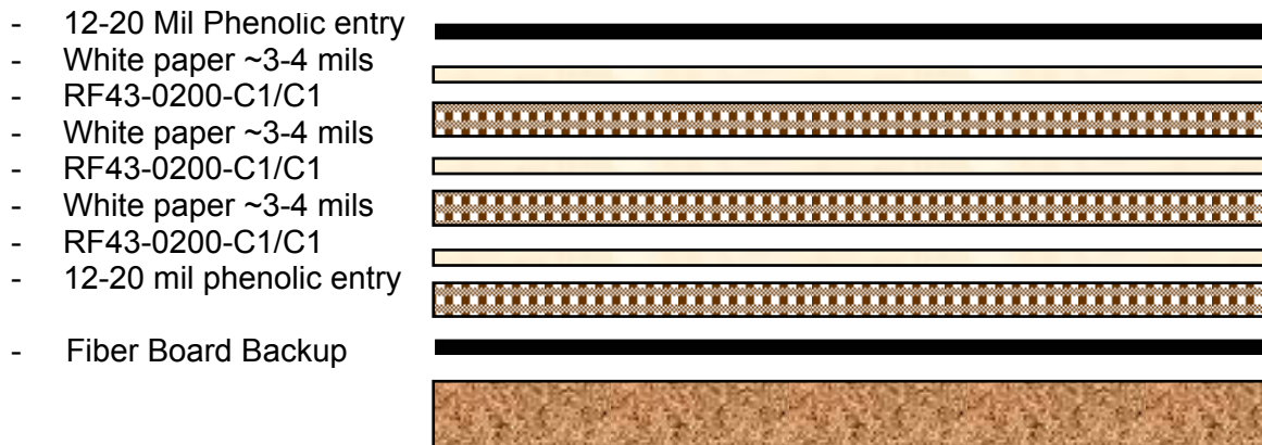
Figure 6 – Typical RF-43 rout stack-up
